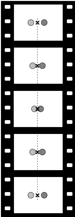
r / The same collision of two pool balls, but now seen in the center of mass frame of reference.
